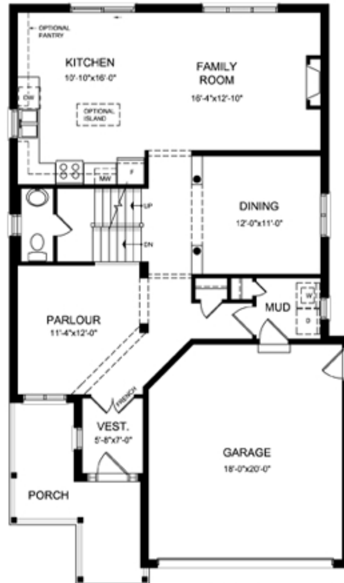
Main Floor Plan 1066 sq. ft.
